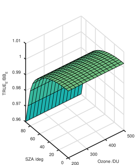
Calibration Matrix fn; Model sdisortREFms2009; f0=1.5542
