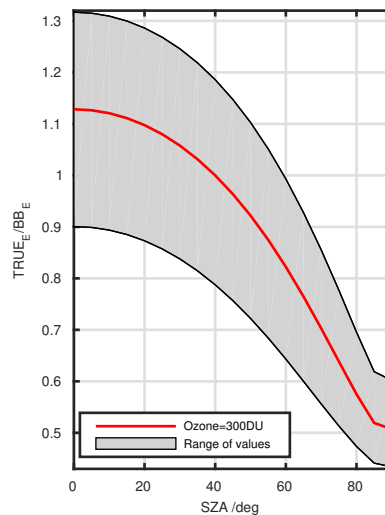
Calibration Matrix fn; Model sdisortREFms2009; f0=0.5373
