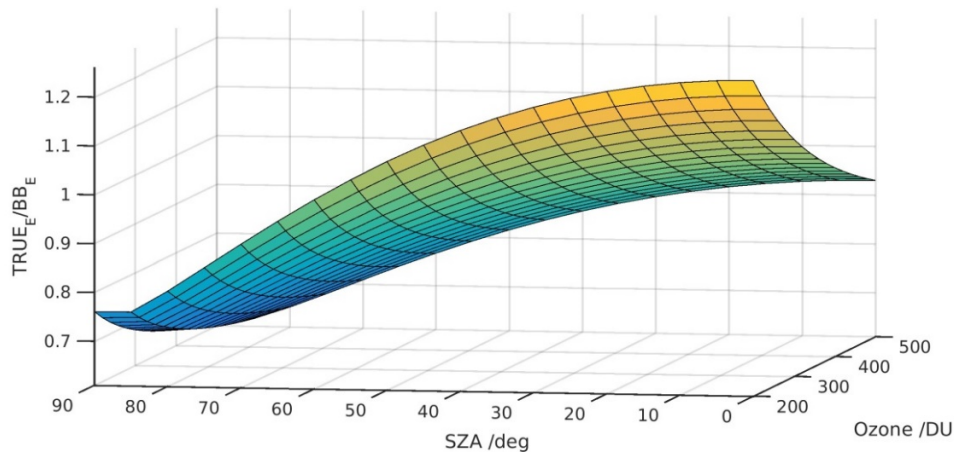
Figure 12. Spectral correction function of a KZ radiometer
