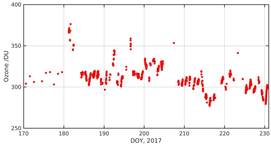
Figure 4. Total ozone column over Davos
