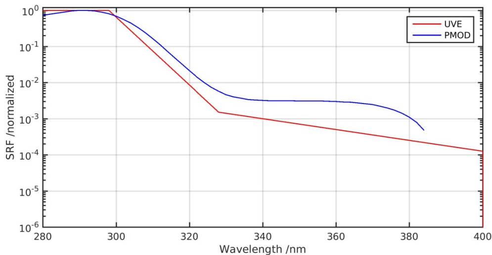
Figure 8. SRF of a KZ radiometer
