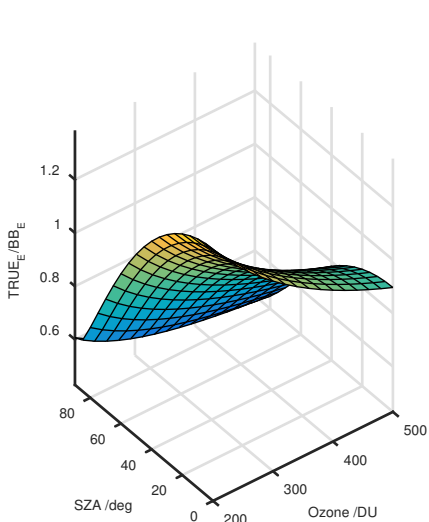
Calibration Matrix fn; Model sdisortREFms2009; f0=0.3430
