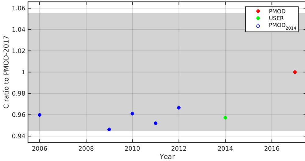
Figure 24. History of the calibration factor C for a SL501 radiometer. The grey shaded area represents the expanded uncertainty of the last calibration factor (red point).
