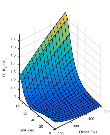
Calibration Matrix fn; Model sdisortREFms2009; f0=0.6230
