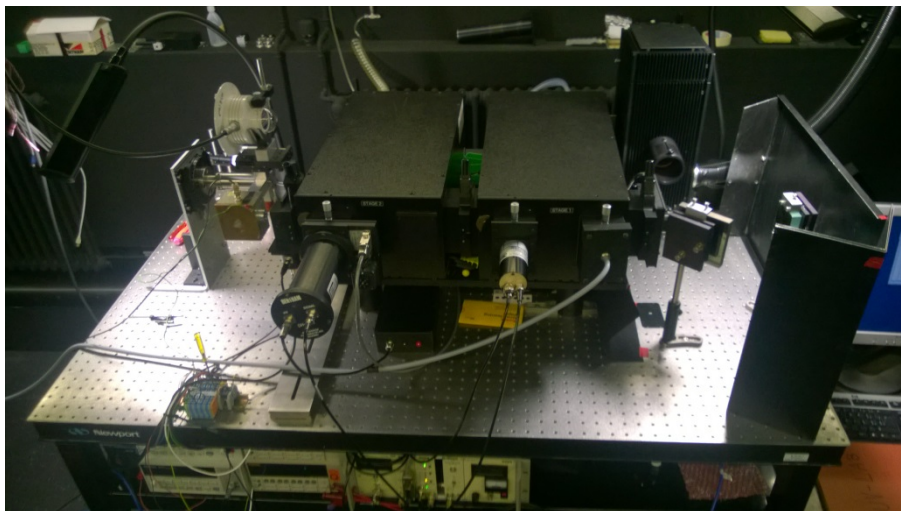
Figure 7. Spectral Response Setup of the WCC-UV
