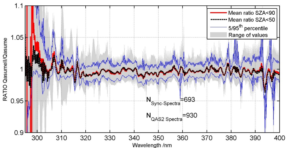
Figure 17. Mean ratio of QASUMEII / QASUME (clear sky data) at PMOD/WRC, 8th April 2017 (098) to 8th October 2017 (281)
