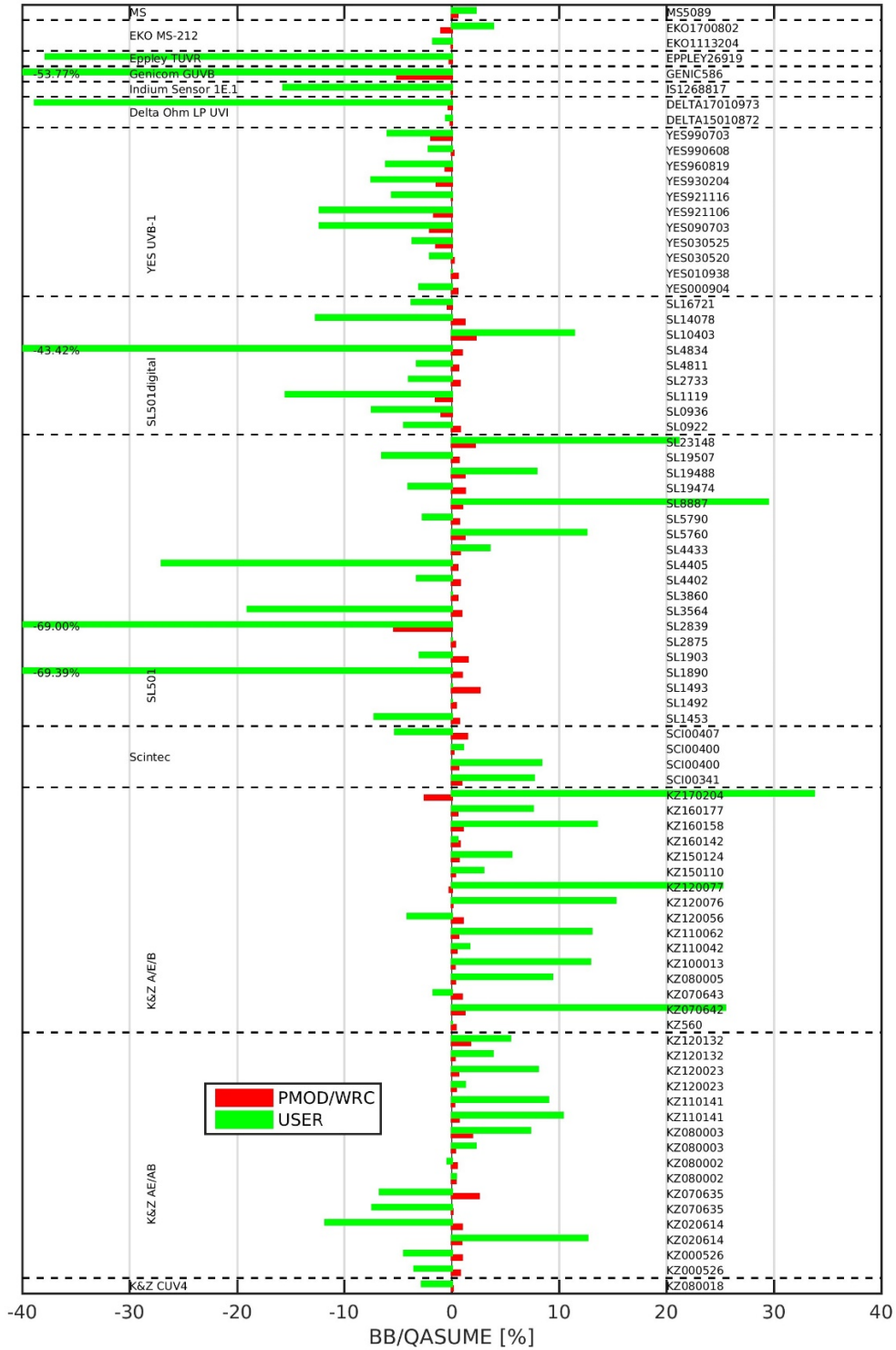
Figure 23. Intercomparison of the original (USER, green) and the new (PMOD, red) calibration
