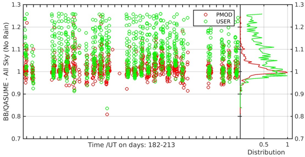
Figure 21. Erythemal weighted broadband irradiance vs. QASUMEII reference data - plotted against the time (left) and as a histogram distribution (right). In this example the data of UVE channel of KZ120023 was used.
