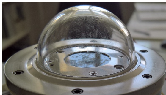
Figure 29. Filter degradation and dome contamination of a YES radiometer
