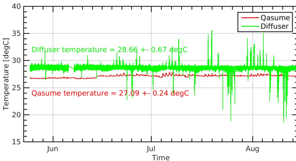
Figure 20. QASUMEII temperature stability of the monochromator and the input optic
