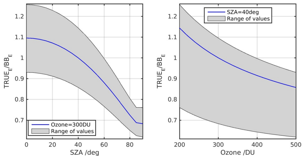
Figure 13. Spectral correction function of a KZ radiometer as projections relative to the SZA (left) and TO_3 (right)
