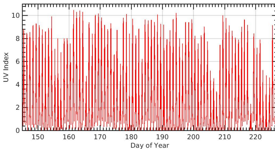
Figure 3. UVI index in Davos, 2017
