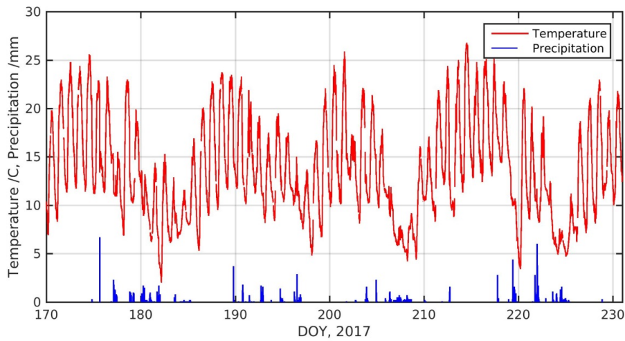
Figure 2. Temperature and precipitation
