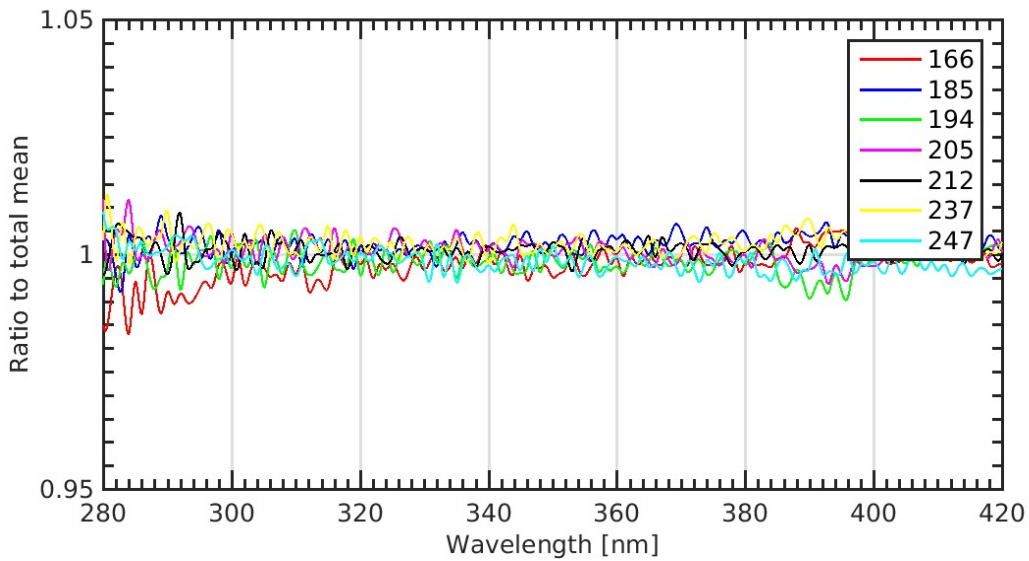
Figure 19. QASUMEII responsivity change based on T68523, 2017
