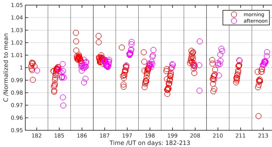
Figure 15. Calibration factors determined for the campaign period for a KZ radiometer. The plots show the inverse of C as defined in the equation above to facilitate the interpretation. A lower calibration factor means a lower signal measured with the radiometer.
