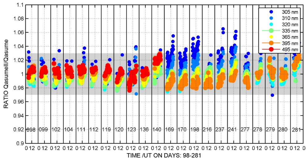
Figure 18. Ratio of QASUMEII / QASUME (clear sky data) at PMOD/WRC, 8th April 2017 (098) to 8th October 2017 (281)
