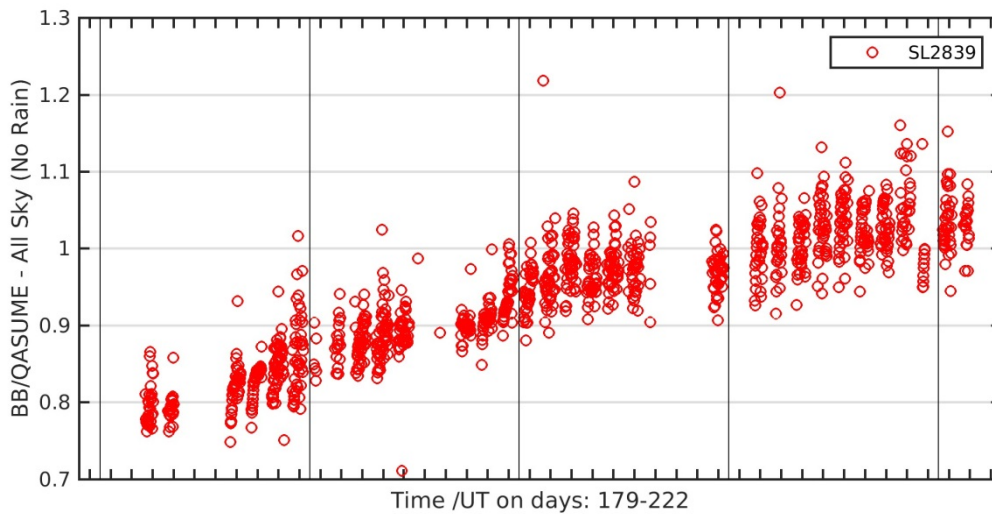
Figure 27. The ratio of the SL2839 irradiance data relative to the reference reveals the sensitivity change after the renewal of the desiccant on DOY 180, 2017.
