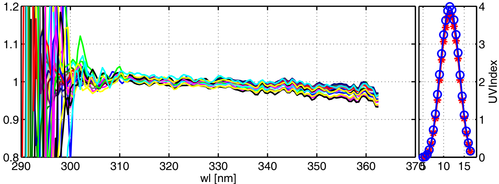
Global irradiance ratios ISQ/JRC at JRC:17-Mar-2004(077)
