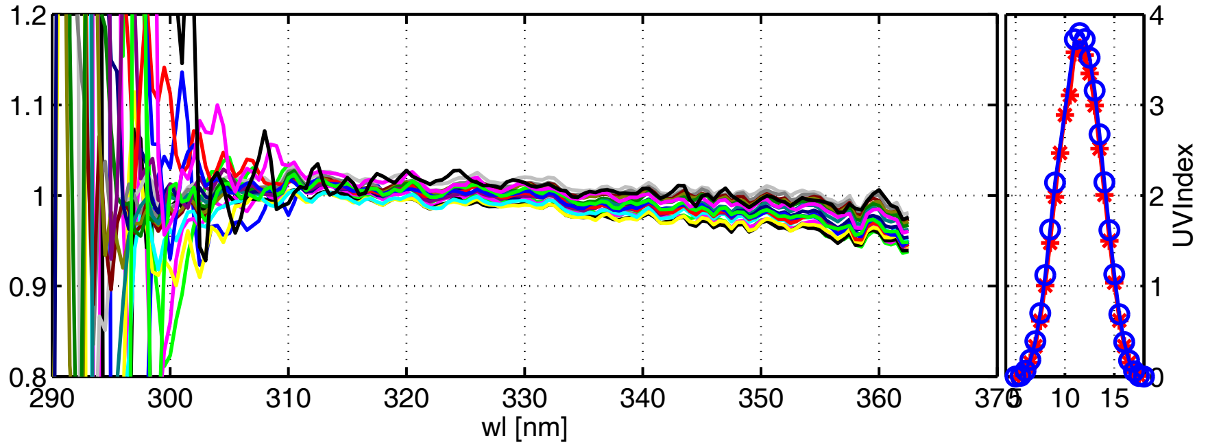
Global irradiance ratios ISQ/JRC at JRC:16-Mar-2004(076)
