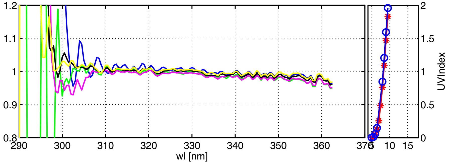
Global irradiance ratios ISQ/JRC at JRC:19-Mar-2004(079)
