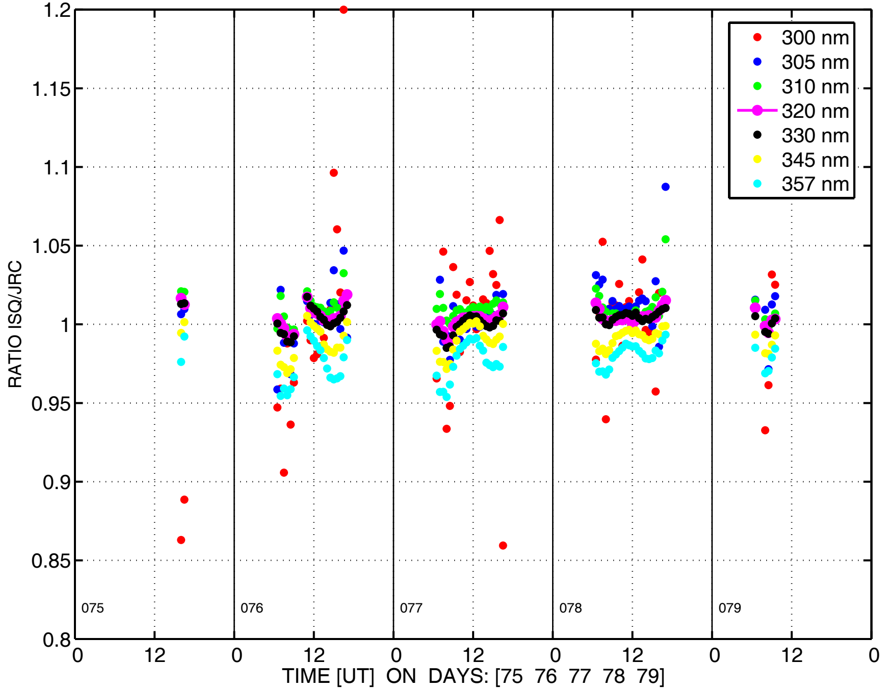
Global irradiance ratios ISQ/JRC at JRC:15-Mar-2004(075) to 19-Mar-2004(079)
