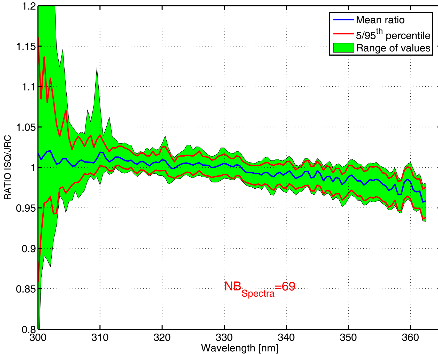
Mean ratio ISQ/JRC at JRC:15-Mar-2004(075) to 19-Mar-2004(079)
