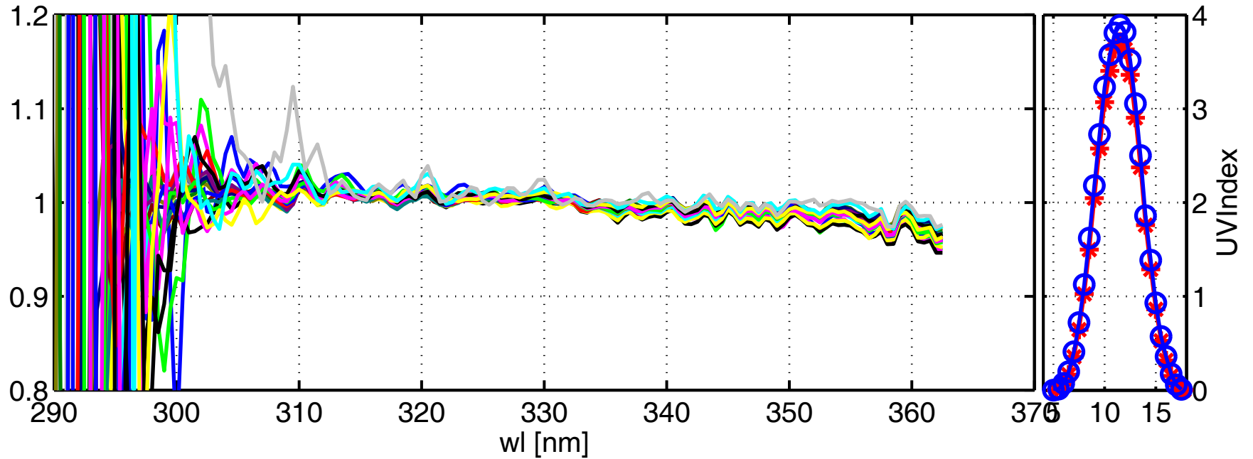
Global irradiance ratios ISQ/JRC at JRC:18-Mar-2004(078)
