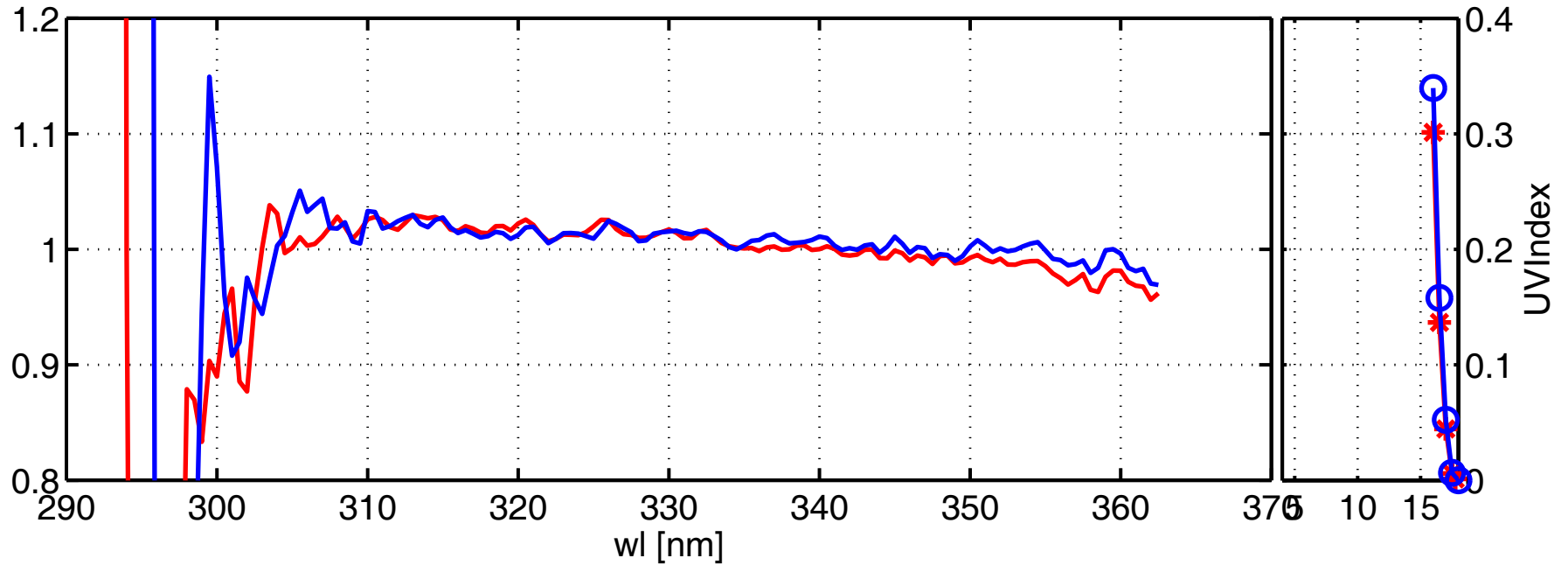
Global irradiance ratios ISQ/JRC at JRC:15-Mar-2004(075)
