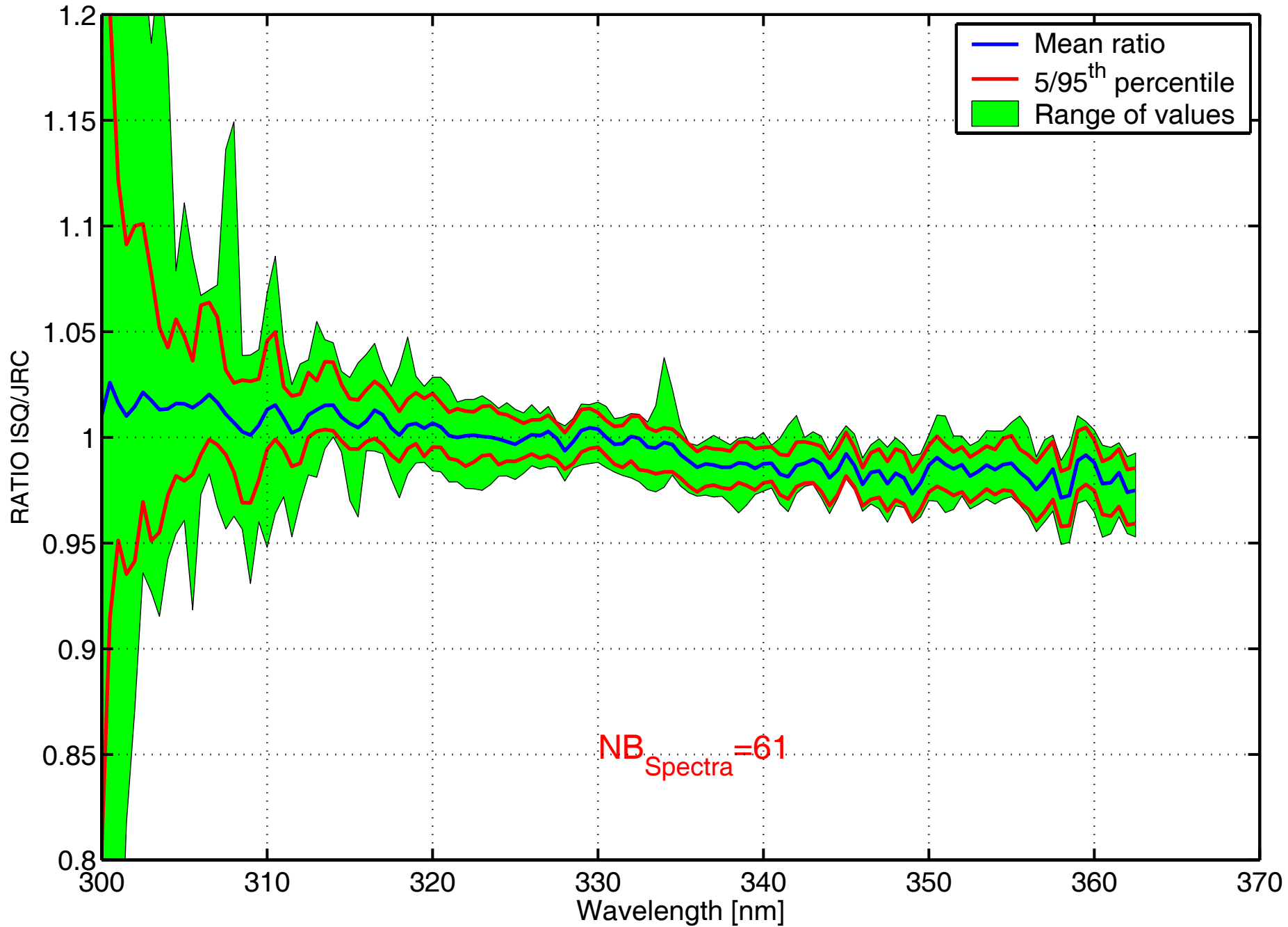
Mean ratio ISQ/JRC at JRC:23-Sep-2003(266) to 26-Sep-2003(269)
